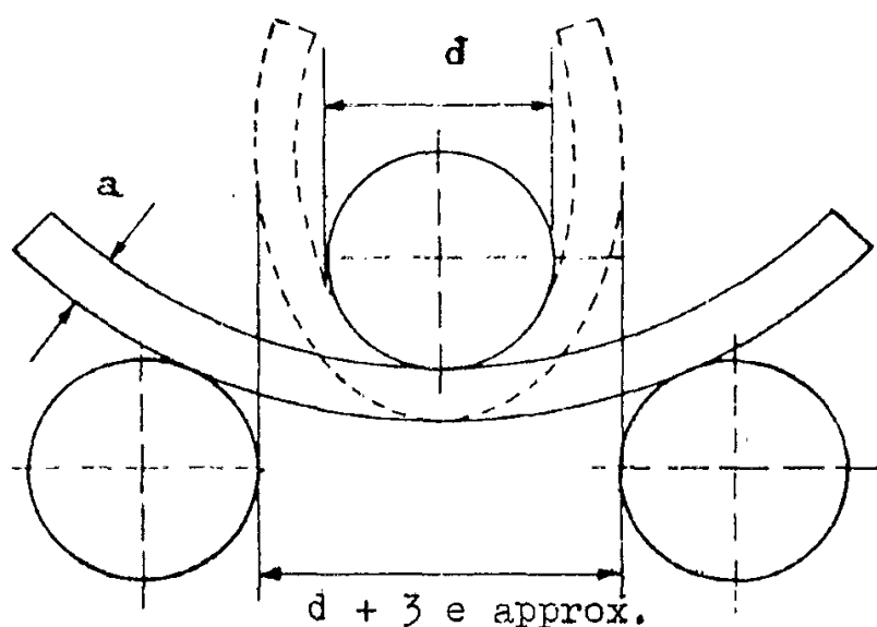
DIAGRAM OF BEND TEST
